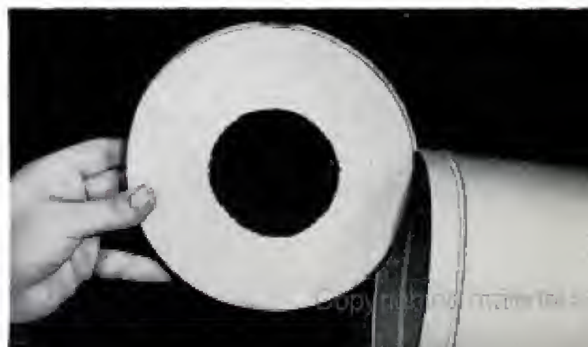
Lower left, No. 1 photoflood bulb gives ample light without excessive heat. Lower right, a hole about 3 in. in dia. in can lid gives fairly sharp spot. Can lid is removed when lamp is used for floodlighting
